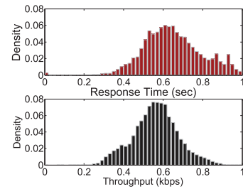
Fig. 8. Transformed distribution.
