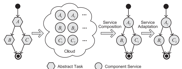
Fig. 2. An example of runtime service adaptation.
