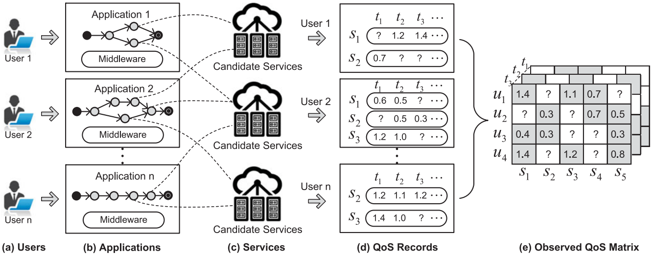
Fig. 4. The problem setting of online QoS prediction.
